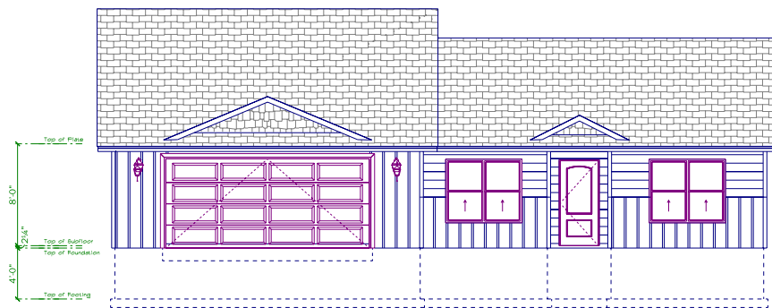
FRONT ELEVATION
