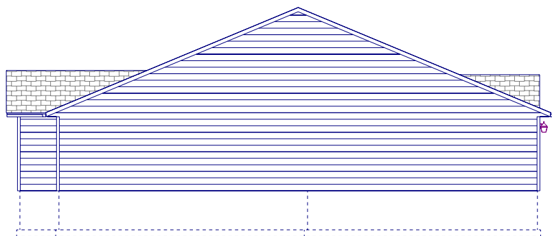
LEFT ELEVATION
